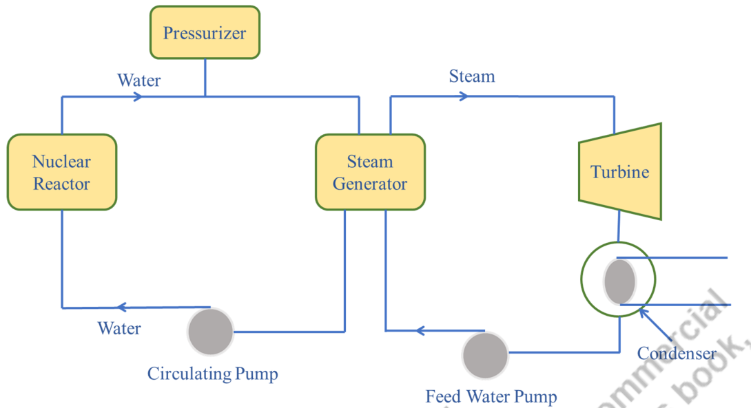
Fig. 5.2. Working of Pressurized Water Reactor
