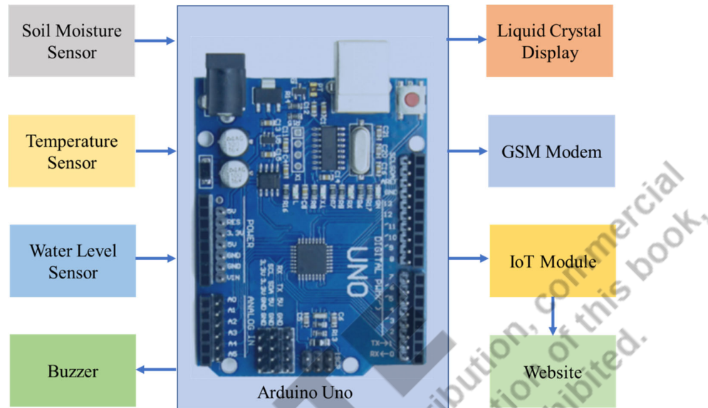
Fig. 4.3. IoT application in coal mining
